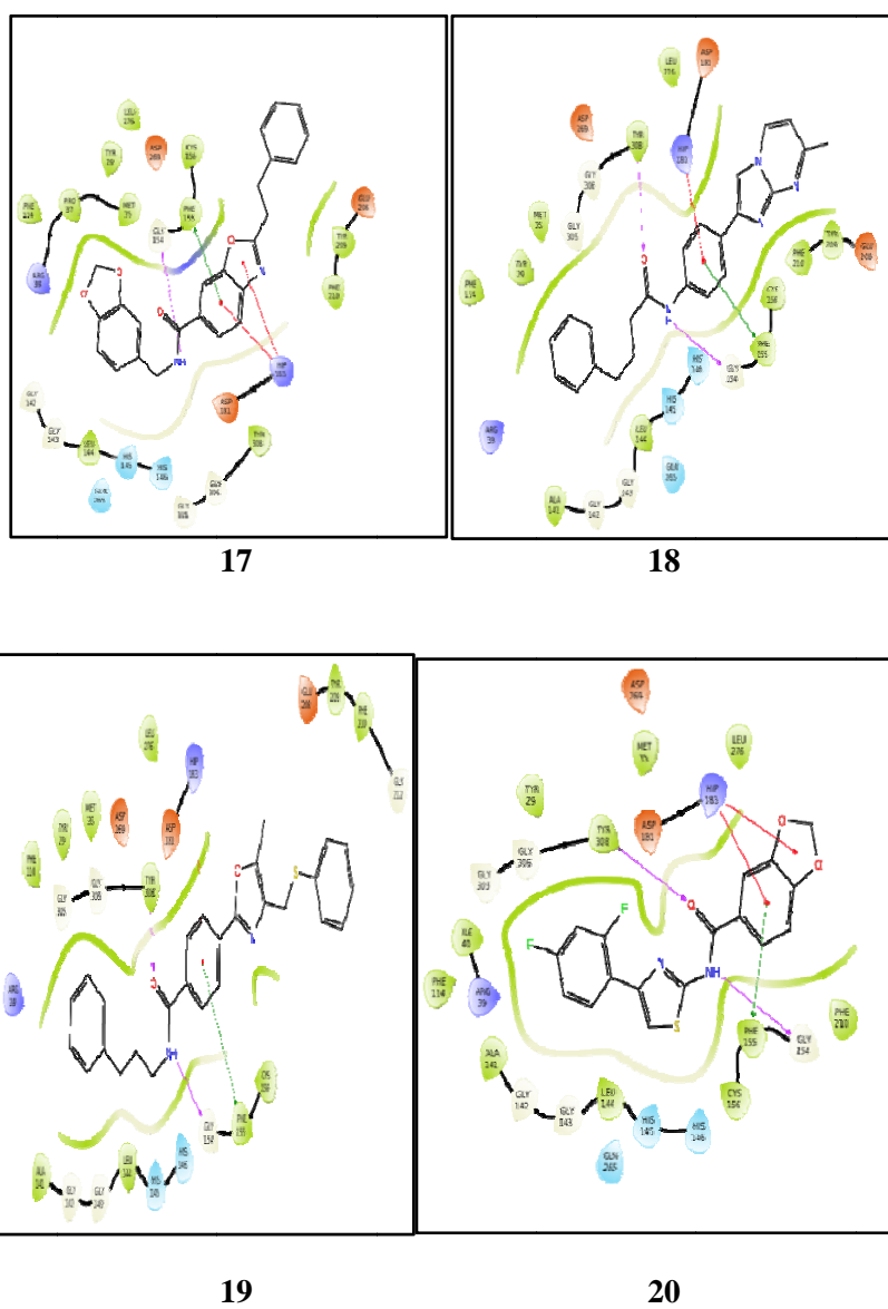
Fig. 1S — 2-D interaction diagram of designed analogs with HDAC (compounds 1-20)
