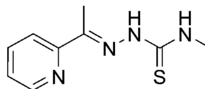
Scheme 1 — Molecular structure of 2-acetylpyridine-N(4)-methyl-3-thiosemicarbazone (L)
