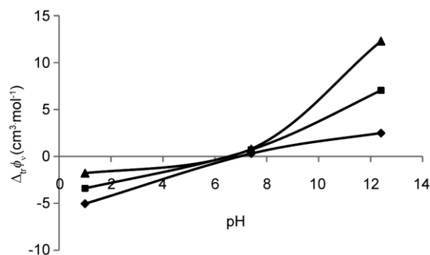
Fig. 1 — Representative plots of limiting partial molar volume of transfer, \Delta_{tr}\phi_v for glycine versus pH in ( \blacklozenge 0.10, \blacksquare 0.50, \blacktriangle 1.00) mol · kg -1 aqueous NaAcB solutions at T(K) = 310.15
