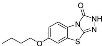
7-Butoxy-2H-benzo[4,5]thiazolo[2,3-c][1,2,4]triazol-3-one (28)
