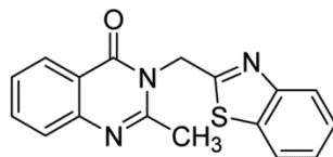
3-Benzothiazol-2-ylmethyl-2-methyl-3H-quinazolin-4-one (30)
