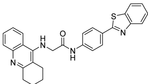
N-(4-Benzothiazol-2-yl-phenyl)-2- (1,2,3,4-tetrahydro-acridin-9-ylamino)-acetamide (40)
