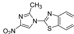
2-(2-Methyl-4-nitro-imidazol-1-yl)-benzothiazole (19)
