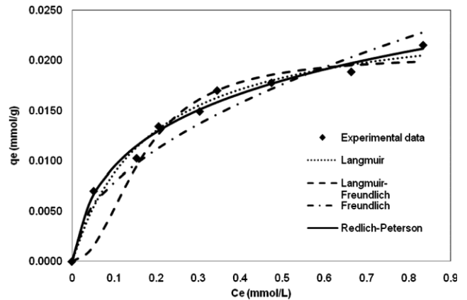
Fig. 6—Equilibrium isotherms of Ni(II) ions on lignin, experimental data and models fit. C_o=5.22-52.22 mg/L Ni; lignin dose = 7g/L; pH=6 ; T=30^\circ C ; solution volume= 25 mL and t=12h .
