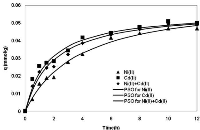
Fig. 5—Kinetic on the binary equilibrium metal uptake in equimolar solution by lignin, experimental data and the best fit, pseudo second order model. Co = 10.44 mg/L Ni, 20 mg/L Cd; lignin dose = 7g/L; solution volume= 25 mL; T= 28°C.
