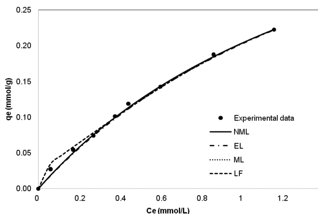
Fig. 11—Equilibrium isotherms of equimolar binary ions on lignin, experimental data and models fit. C_0=5.22-52.22 mg/L Ni, 10-100 mg/L Cd; dose sample= 7g/L; pH=6 ; T=40^\circ\text{C} ; solution volume= 25 mL and t=12 h.
