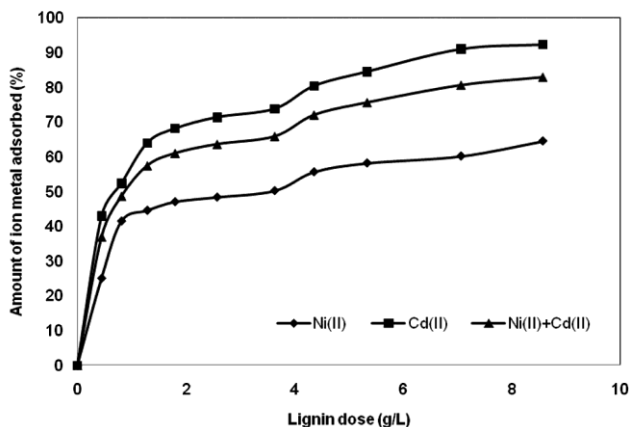
Fig. 2—Effect of lignin dose on the binary equilibrium metal uptake for equimolar solution. C_0 = 10.44 mg/L Ni, 20 mg/L Cd; solution volume = 25 mL; pH=6 ; T=28^\circ\text{C} and t = 8 h.
