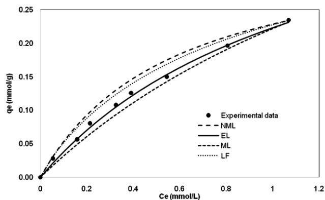
Fig. 10—Equilibrium isotherms of equimolar binary ions on lignin, experimental data and models fit. C_0=5.22-52.22 mg/L Ni, 10-100 mg/L Cd; dose sample= 7g/L; pH=6 ; T=30^\circ\text{C} ; solution volume= 25 mL and t=12 h.
