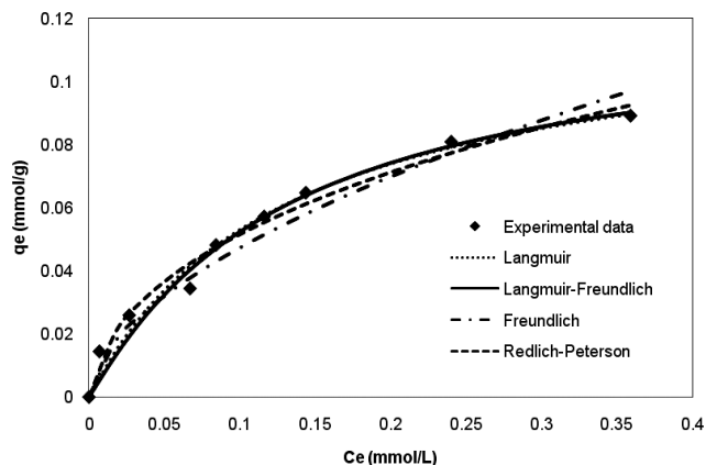
Fig. 9—Equilibrium isotherms of Cd(II) ions on lignin, experimental data and models fit. C_0=10-100 mg/L Cd; lignin dose = 7g/L; pH=6 ; T=40^\circ\text{C} ; solution volume= 25 mL and t=12 h.
