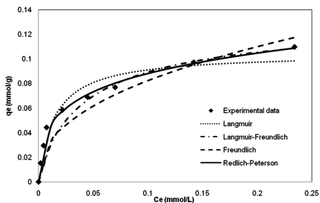
Fig. 8—Equilibrium isotherms of Cd(II) ions on lignin, experimental data and models fit. C_0=10-100 mg/L Cd; lignin dose = 7g/L; pH=6 ; T=30^\circ\text{C} ; solution volume= 25 mL and t=12 h.
