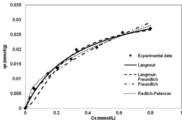
Fig. 7—Equilibrium isotherms of Ni(II) ions on lignin, experimental data and models fit. C_0=5.22-52.22 mg/L Ni; lignin dose = 7g/L; pH=6 ; T=40^\circ\text{C} ; solution volume= 25 mL and t=12 h.
