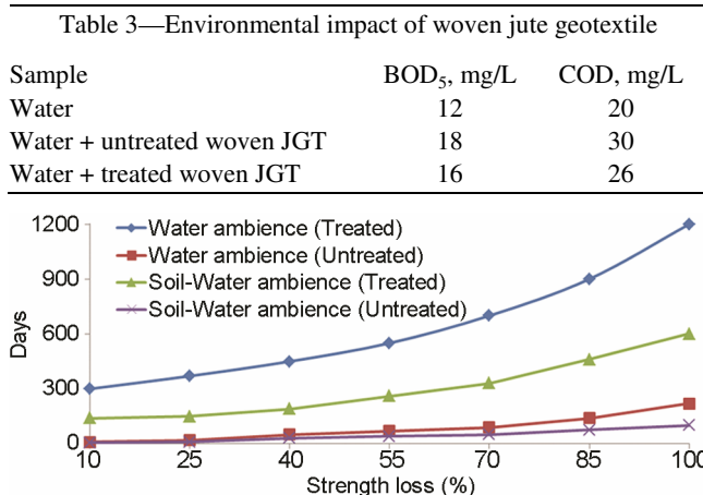
Fig. 2—Statistical life prediction of treated woven jute geotextile
