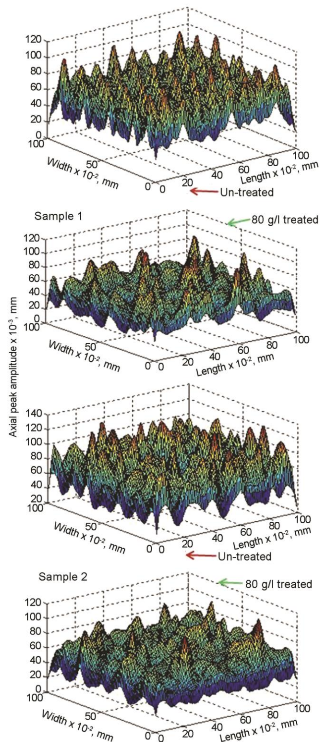
Fig. 2 — Surface plots obtained by DIP method for untreated and 80 g/L silicone treated handloom fabrics (Samples 1 and 2)
