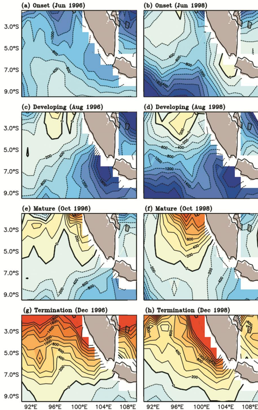
Fig. 6 — Ekman transport ( \text{kg m}^{-1} \text{s}^{-1} ) in the eastern box [90E:110E; 10S: EQ] during the pure negative IOD (1996) and La-Nina-negative IOD co-occurred event (1998) for the different phases of evolution
