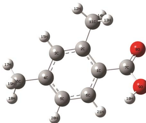
Fig. 1 — Molecular structure of 2,4-dimethylbenzoic acid along with numbering of atoms.
