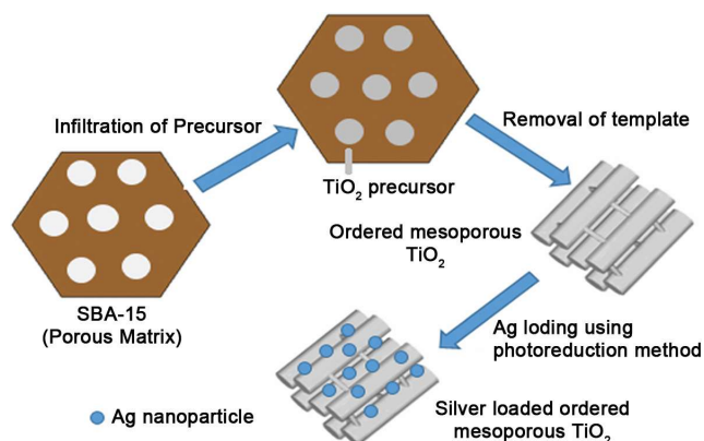
Fig. 1 — Schematic illustration of the synthesis of SMTO material.
