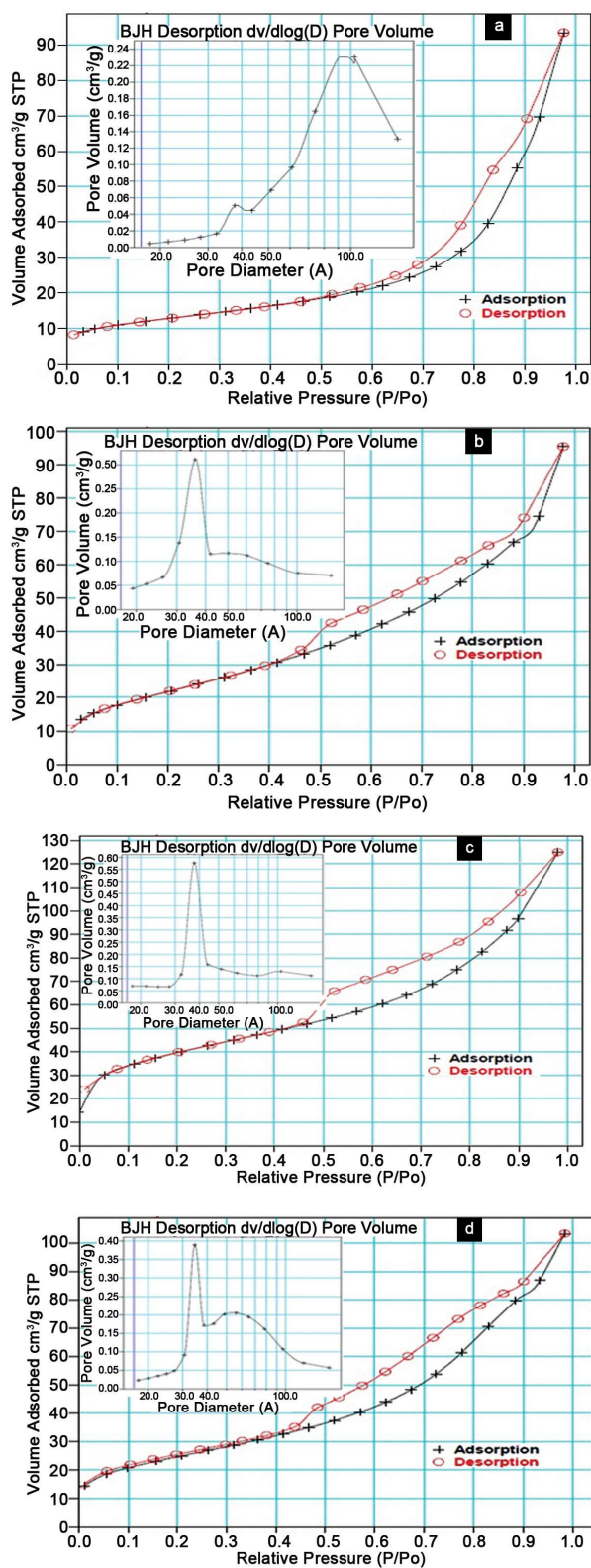
Fig. 4 — (a,d) N 2 adsorption-desorption isotherms for Ag=0, 1.0, 2.0 and 3.0 SMTO materials, respectively. Their corresponding BJH pore size distribution is shown in inset of respective figures.
