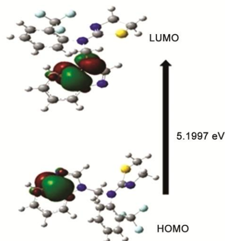
Fig. 4 — HOMO-LUMO molecular orbital of the title compound.
