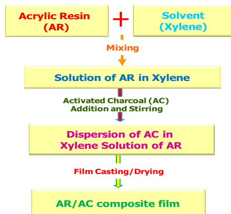
Fig. 1 — Schematic representation of formation of AC/AR composites by solution processing route
