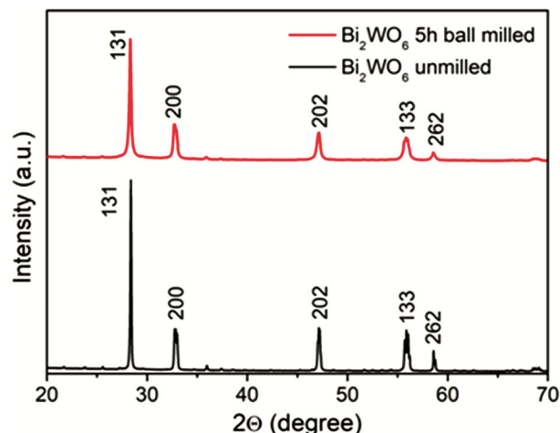
Fig. 1 — XRD diffractogram of Bi 2 MoO 6 unmilled and 5h ball-milled.
