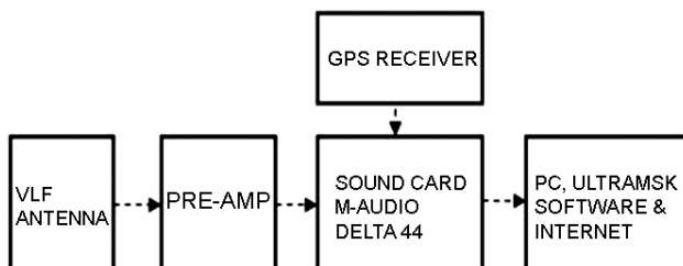
Fig. 1 — Block diagram of the VLF receiver
