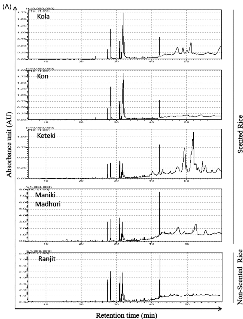
Fig. 1 — GCMS fingerprinting analysis: (A) GCMS fingerprinting was recorded for all the indicated rice varieties with a 30 m x 0.25 \mu m x 0.25 mm EB-5 MS capillary column in a same concentration.
