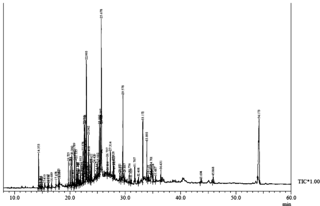
Fig. 2 — Chromatogram of AIA3 isolate showing peaks of compounds in GCMS analysis
