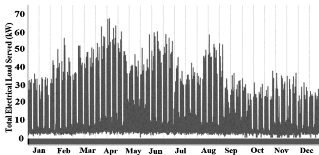
Fig. 12 — Annual power served to the load by optimum-1 system
