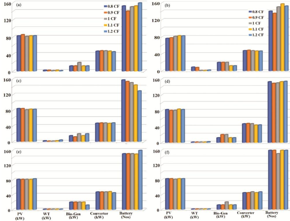
Fig. 13 — HRES Optimization on varying cost factor of (a) solar PV, (b) wind turbine, (c) battery, (d) converter, (e) bio-gen, and (f) fuel from 0.8 to 1.2
