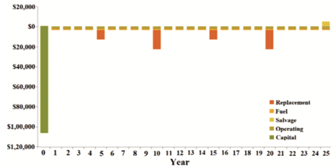
Fig. 9 — Flow analysis of total cost for optimum-1 system
