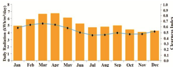
Fig. 2 — Solar resource availability at selected site 26
