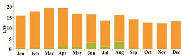
Fig. 11 — Monthly average power generation from the optimum-1 system
