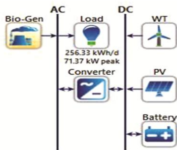
Fig. 1 — Hybrid system model designed in Homer Pro
