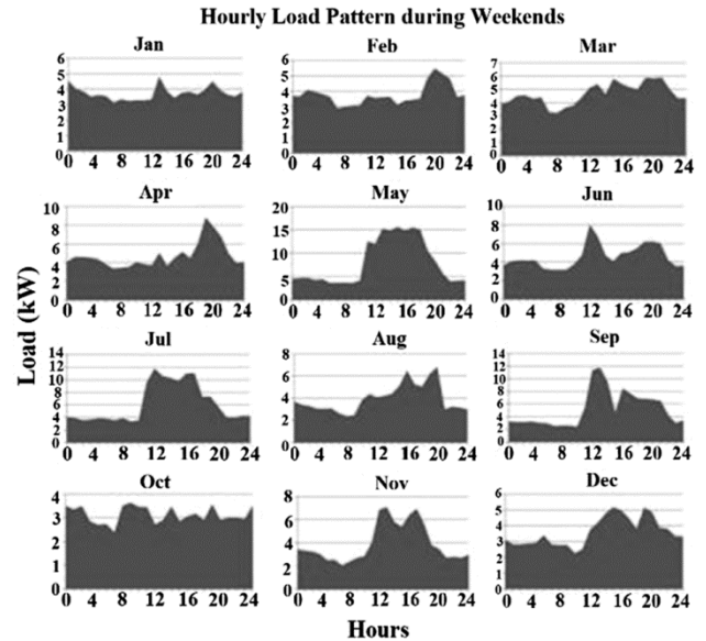
Fig. 7 — Monthly based hourly loading pattern during weekends for the year 2019
