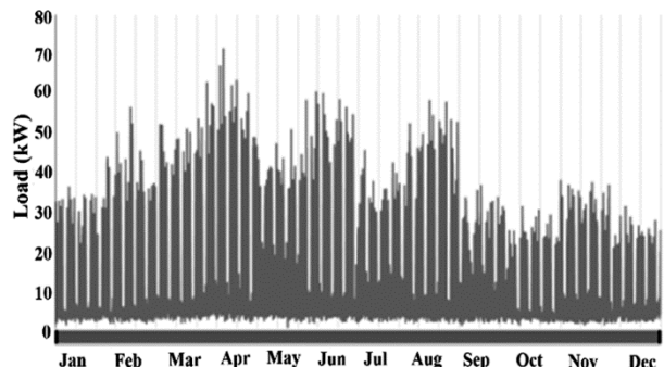
Fig. 5 — Institutional load demand pattern over full year
