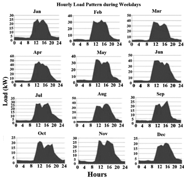
Fig. 6 — Monthly based hourly loading pattern during weekdays for the year 2019
