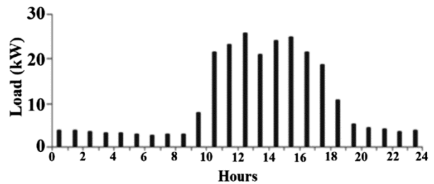
Fig. 4 — Institutional hourly-wise average load pattern
