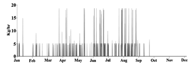
Fig. 10 — Fuel consumption on bio-generator of optimum-1
