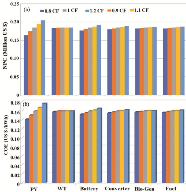
Fig. 14 — Effect on (a) NPC, and (b) COE upon variation of cost factor of solar PV, wind turbine, battery, bio-gen and fuel from 0.8 to 1.2
