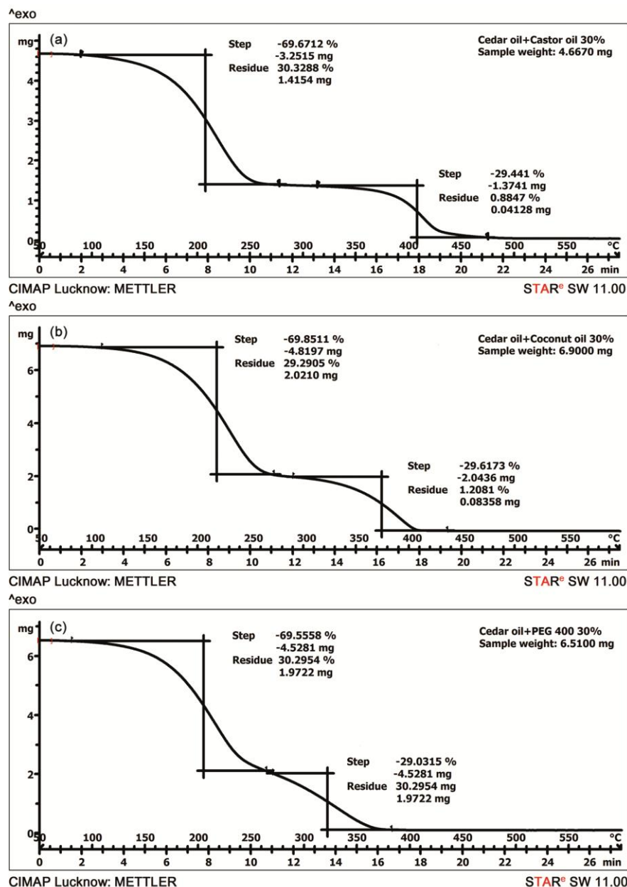
Fig. 5 — The representative TGA pattern for adulterated sample comprising of 70% cedarwood oil and 30% of (A) Castor Oil, (B) Coconut Oil, and (C) PEG-400
