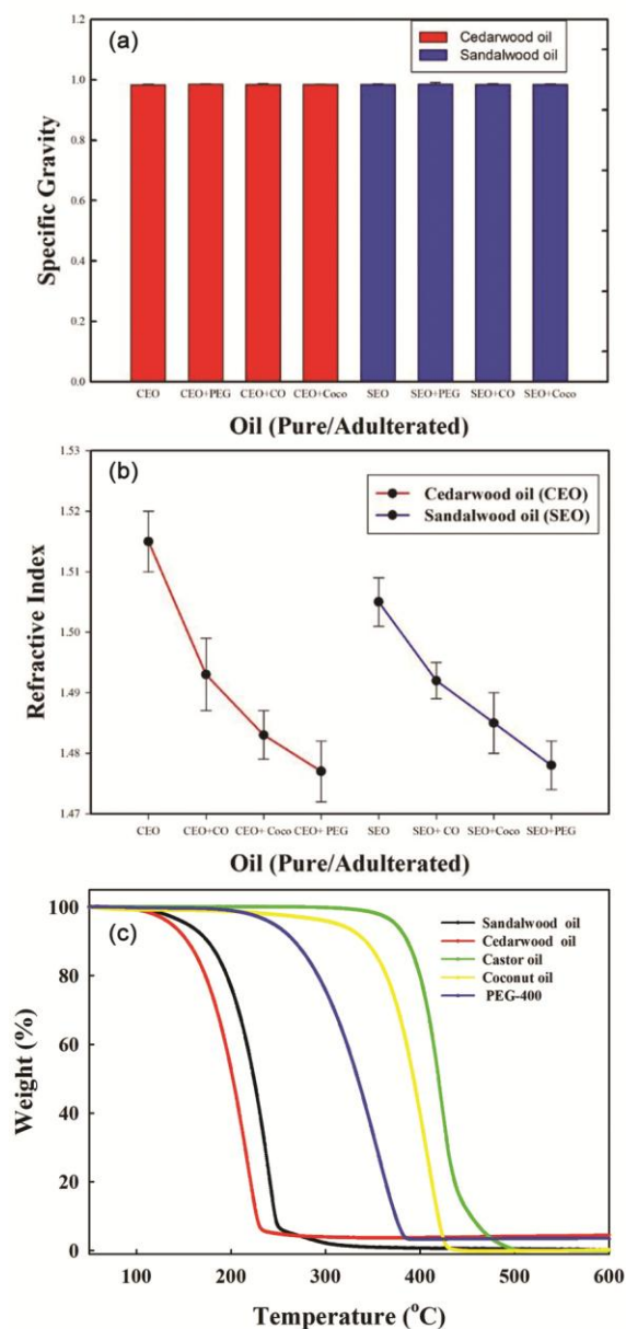
Fig. 1 — Pure and adulterated sandalwood and cedarwood essential oil: (A) specific gravity, (B) Refractive index, (C) TGA of essential oil, vegetable oil, and PEG-400 (CO = Castor Oil, Coco = Coconut Oil, PEG-400 = Polyethylene glycol-400)
