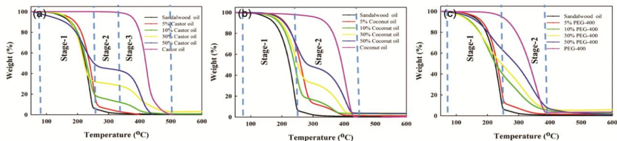
Fig. 2 — Comparison of TGA patterns of sandalwood oil: pure, and adulterated using 5%, 10%, 30% and 50% of (A) Castor Oil, (B) Coconut Oil, and (C) PEG-400
