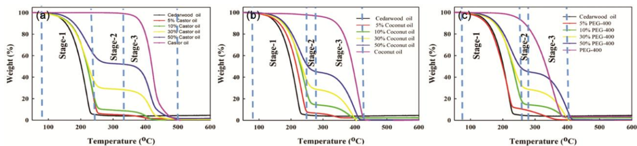
Fig. 4 — Comparison of TGA patterns of cedarwood oil: pure, and adulterated using 5%, 10%, 30% and 50% of (A) Castor Oil, (B) Coconut Oil, and (C) PEG-400
