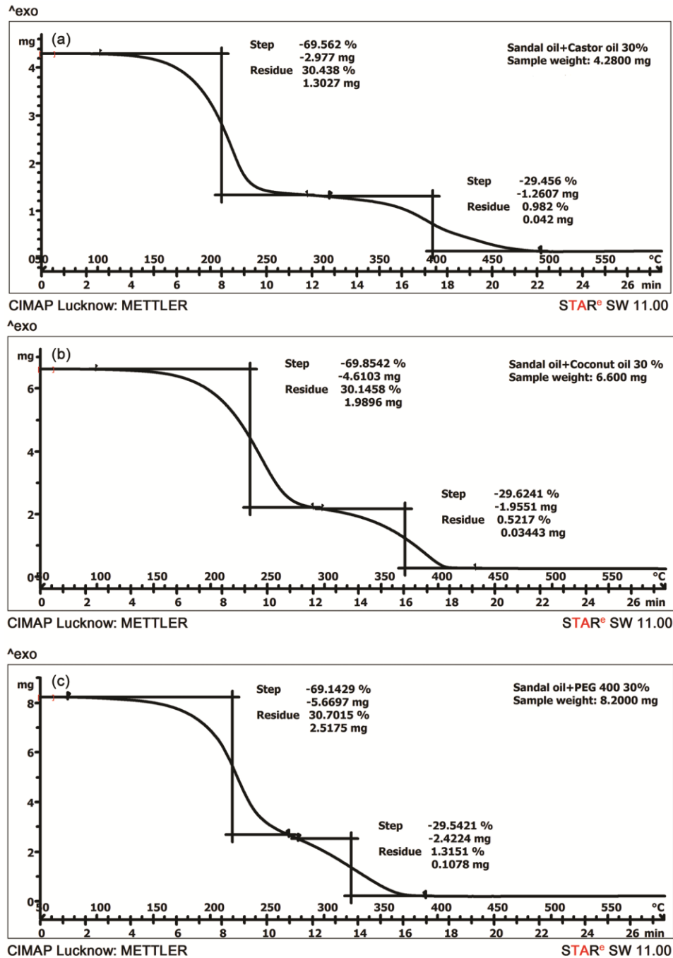
Fig. 3 — The TGA pattern for adulterated sample comprising of 70% sandalwood oil and 30% of (A) Castor Oil, (B) Coconut Oil, and (C) PEG-400
